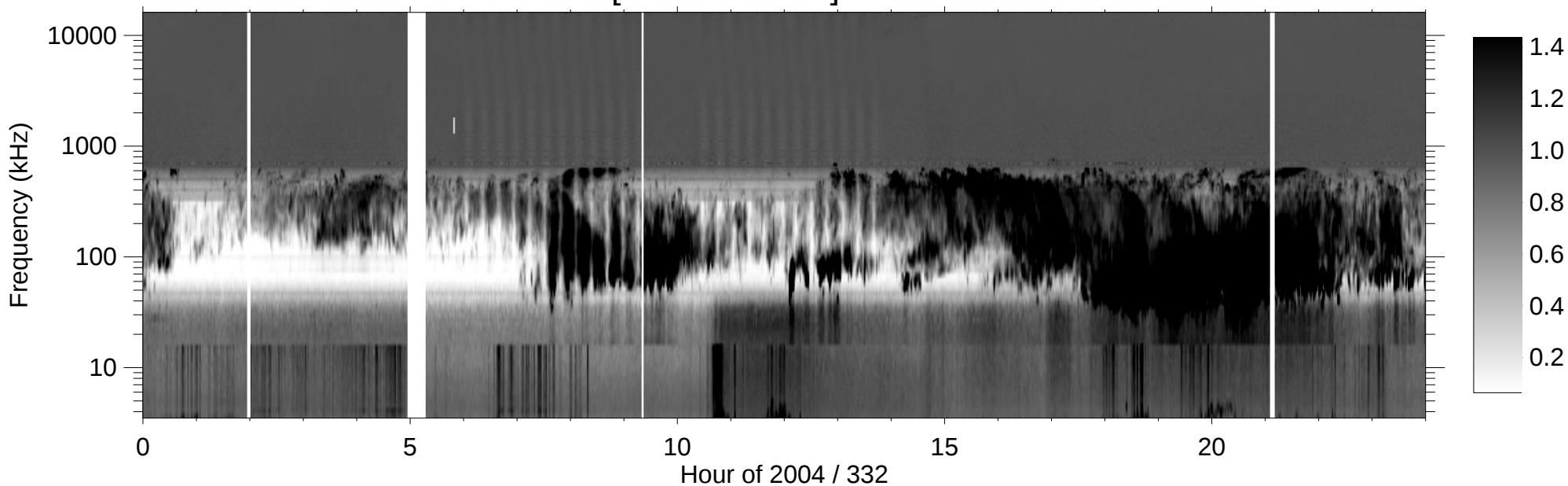
RPWS [ABCH1H2/Ex] (-B) 2004/11/27
