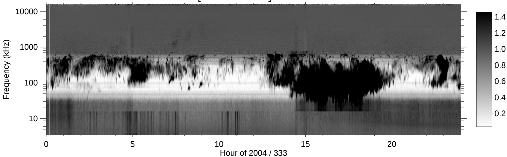
RPWS [ABCH1H2/Ex] (-B) 2004/11/28
