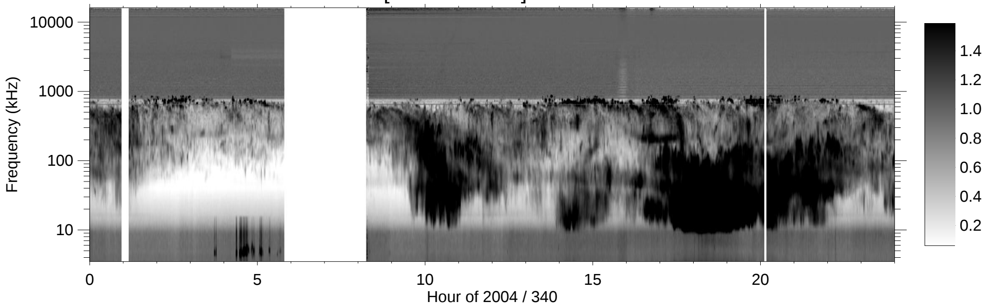
RPWS [ABCH1H2/Ex] (-B) 2004/12/05
