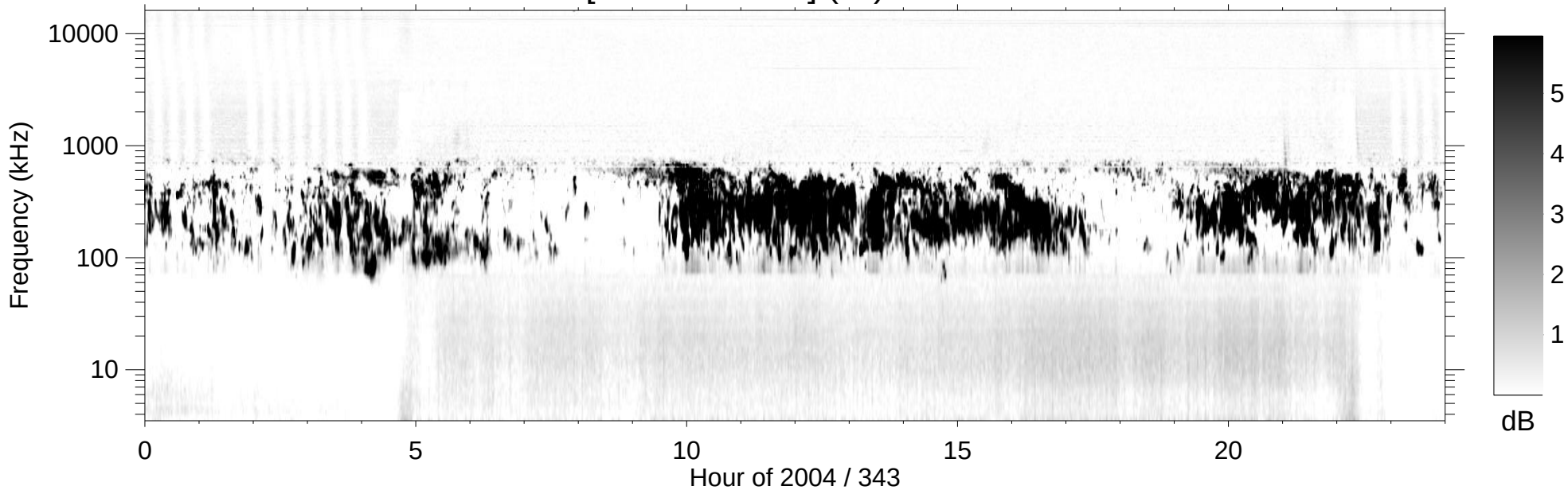
RPWS [ABCH1H2/Ex] (-B) 2004/12/08
