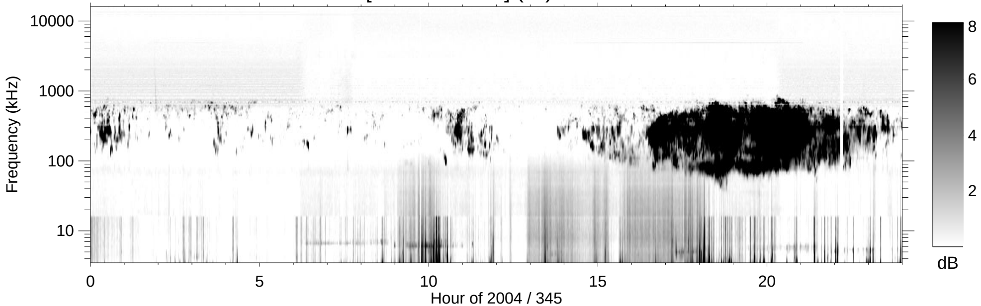
RPWS [ABCH1H2/Ex] (-B) 2004/12/10
