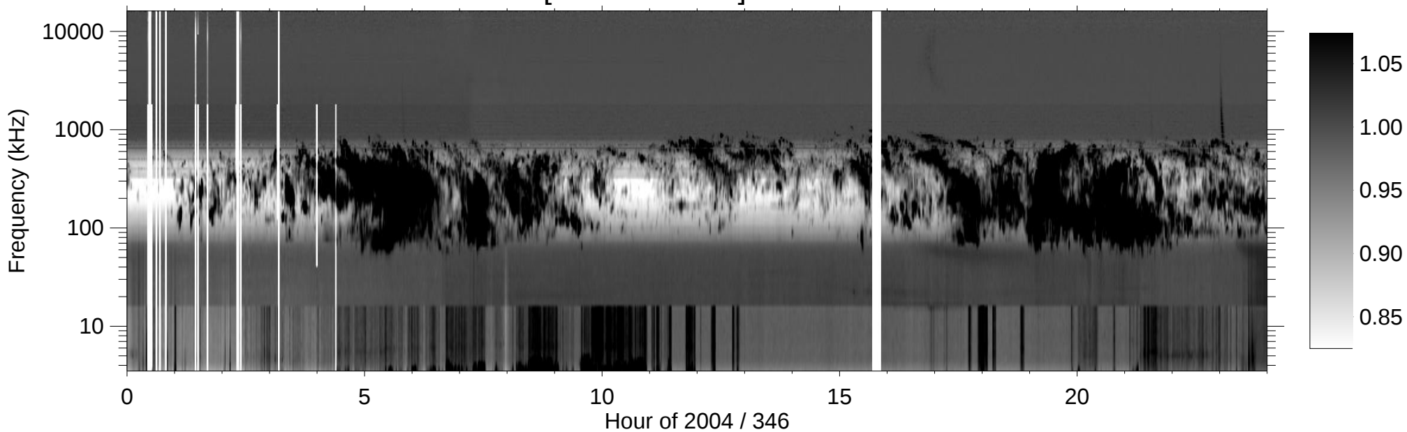
RPWS [ABCH1H2/Ex] (-B) 2004/12/11
