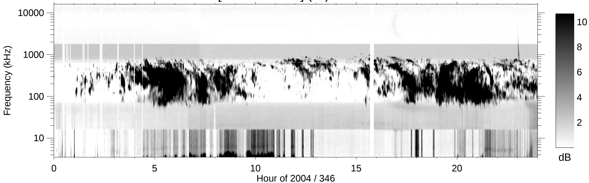
RPWS [ABCH1H2/Ex] (-B) 2004/12/11
