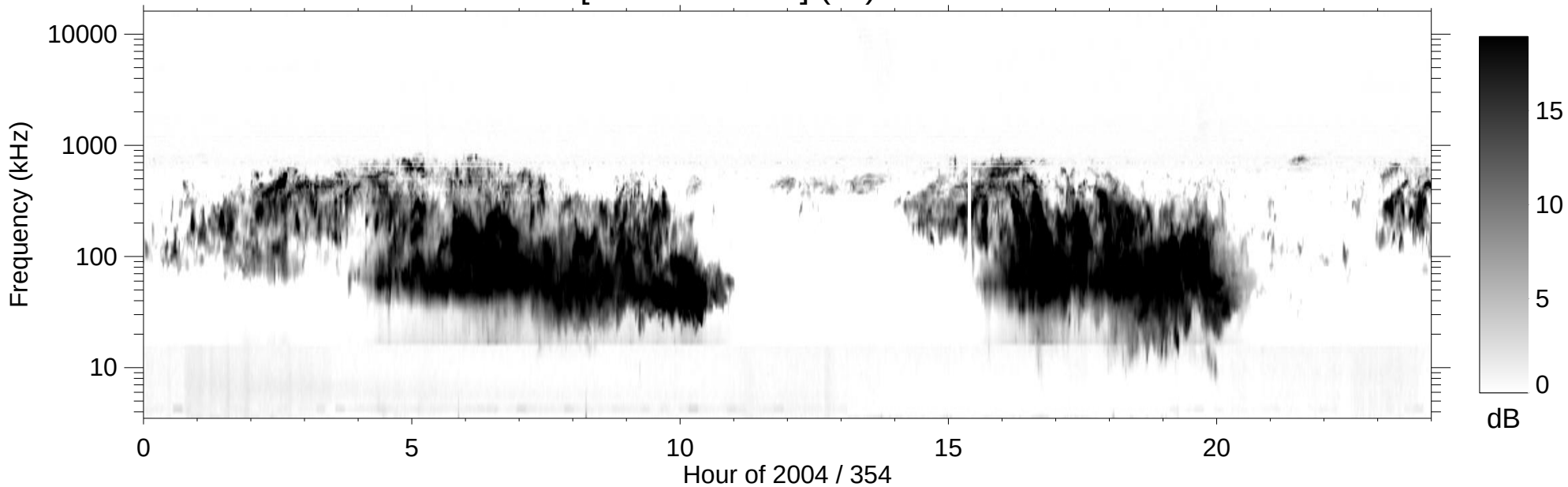
RPWS [ABCH1H2/Ex] (-B) 2004/12/19
