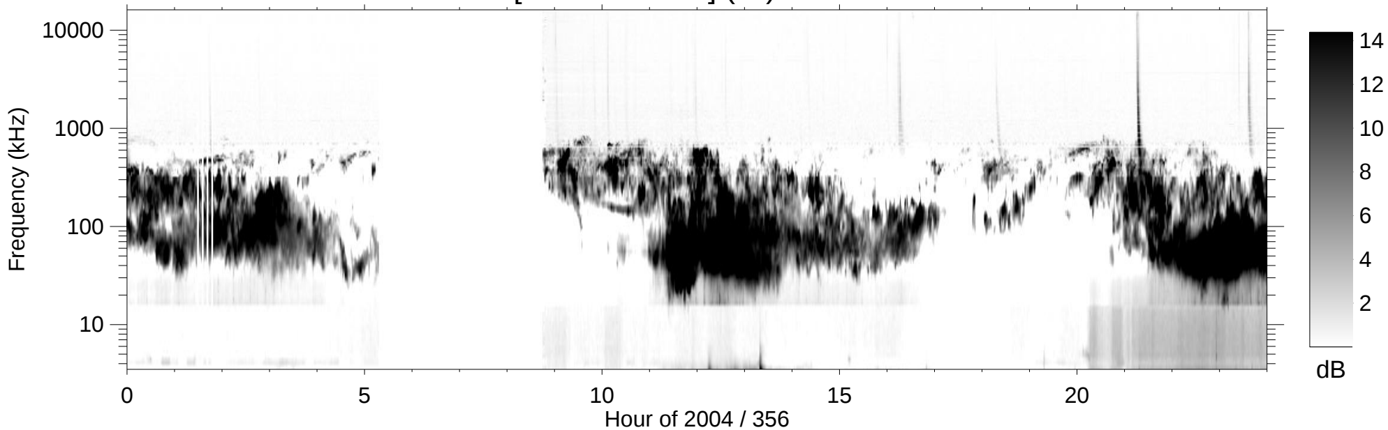
RPWS [ABCH1H2/Ex] (-B) 2004/12/21
