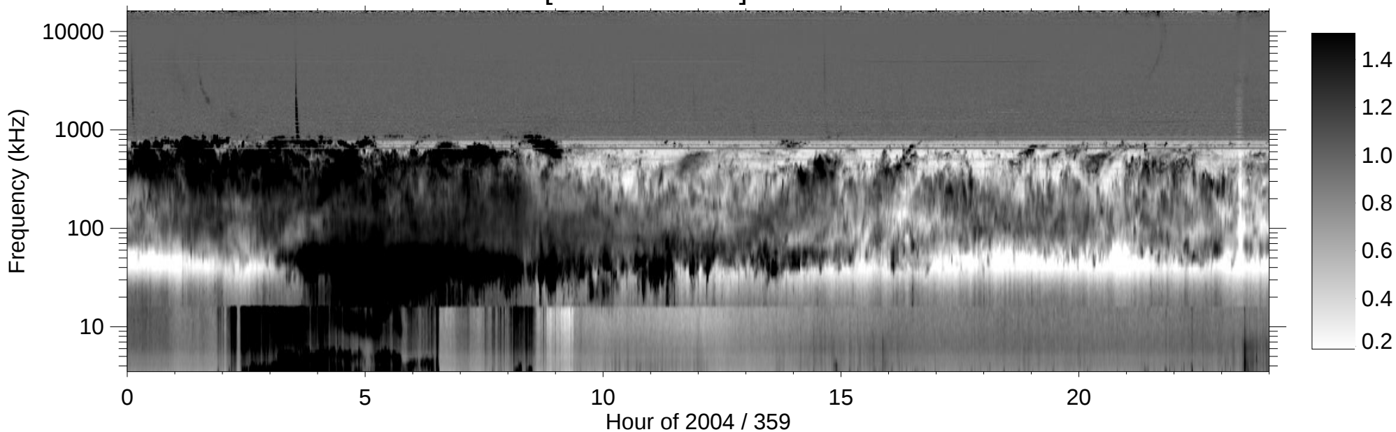
RPWS [ABCH1H2/Ex] (-B) 2004/12/24
