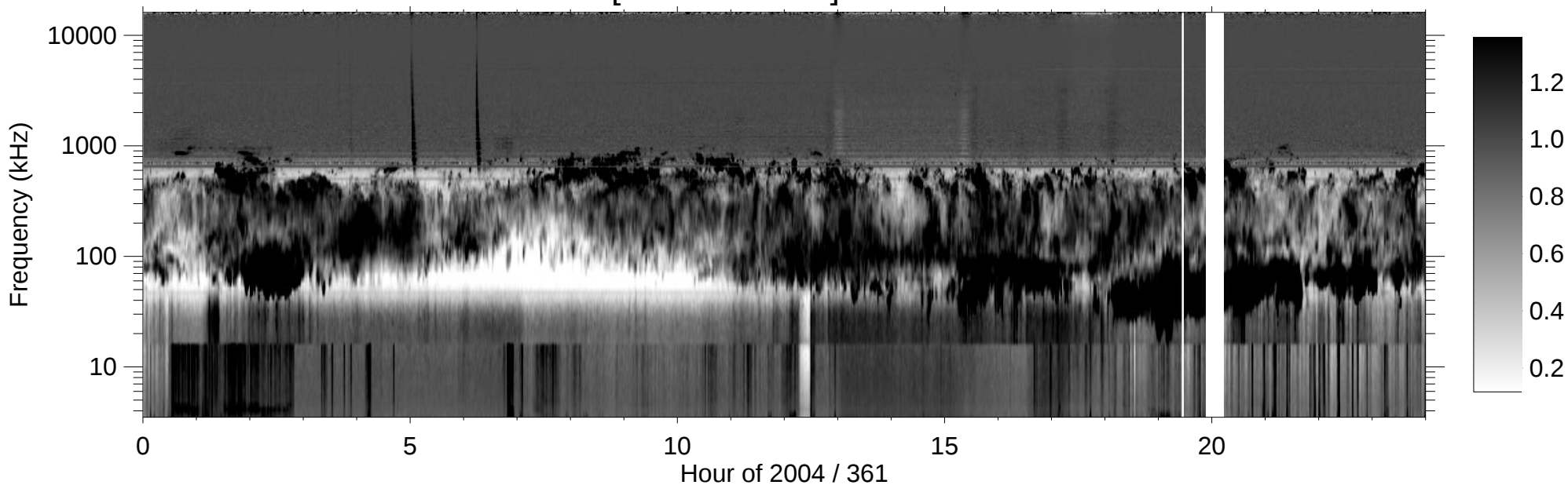
RPWS [ABCH1H2/Ex] (-B) 2004/12/26
