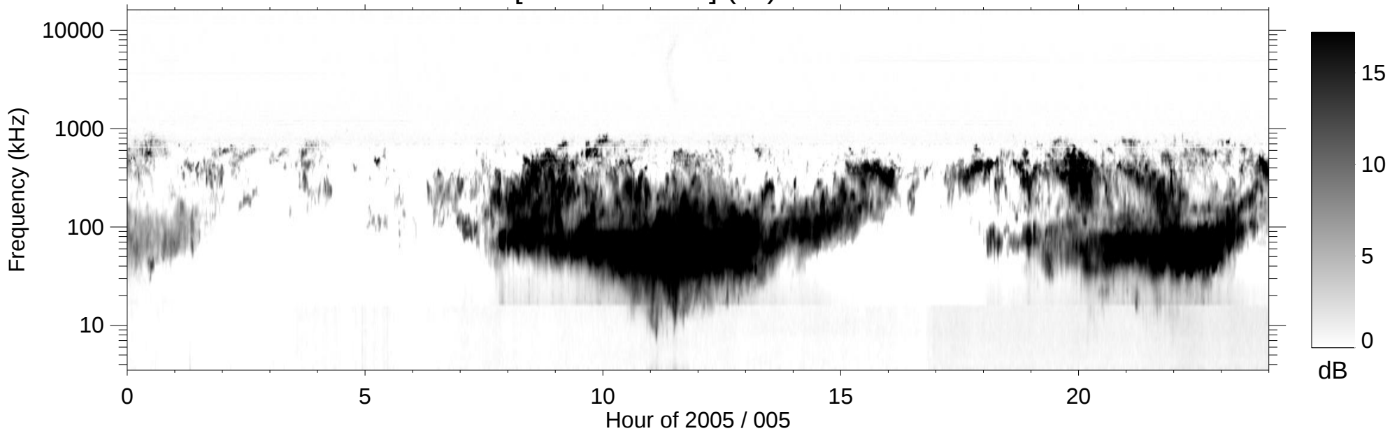
RPWS [ABCH1H2/Ex] (-B) 2005/01/05
