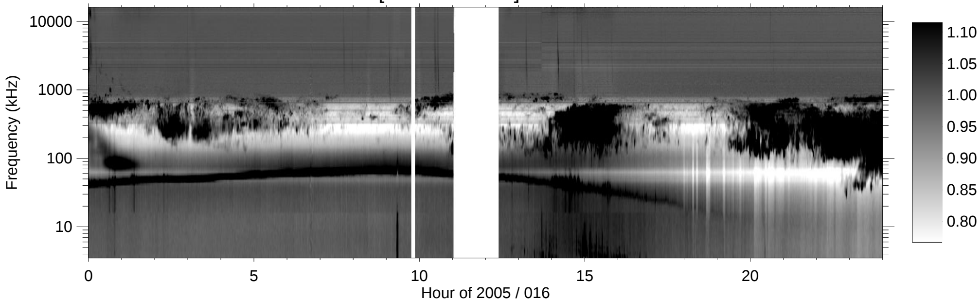
RPWS [ABCH1H2/Ex] (-B) 2005/01/16
