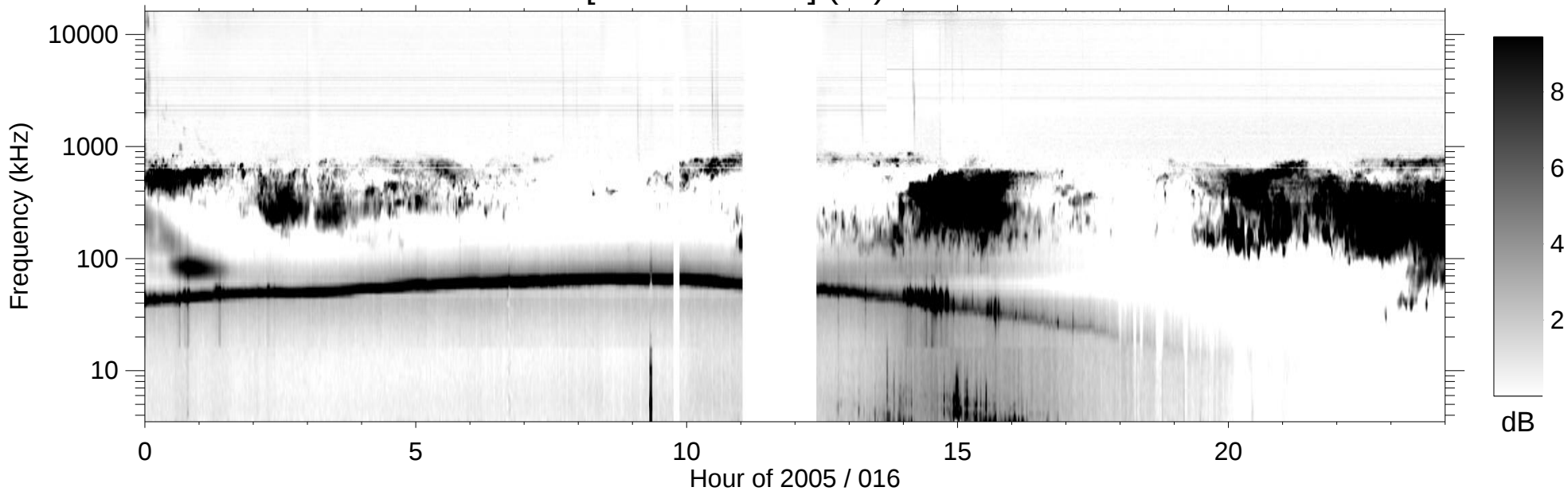
RPWS [ABCH1H2/Ex] (-B) 2005/01/16
