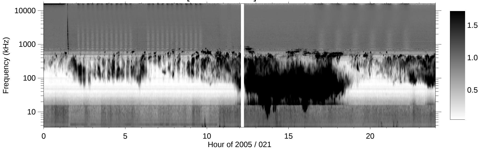
RPWS [ABCH1H2/Ex] (-B) 2005/01/21
