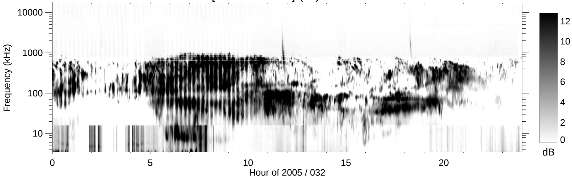
RPWS [ABCH1H2/Ex] (-B) 2005/02/01
