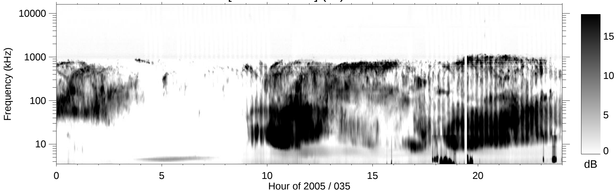
RPWS [ABCH1H2/Ex] (-B) 2005/02/04
