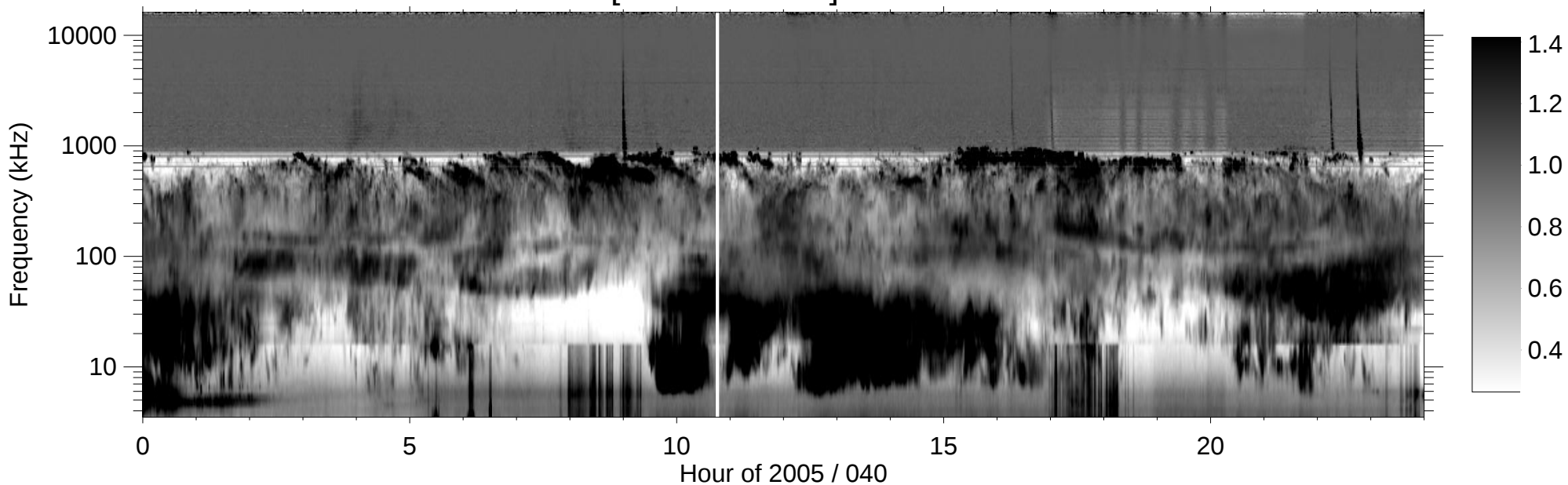
RPWS [ABCH1H2/Ex] (-B) 2005/02/09
