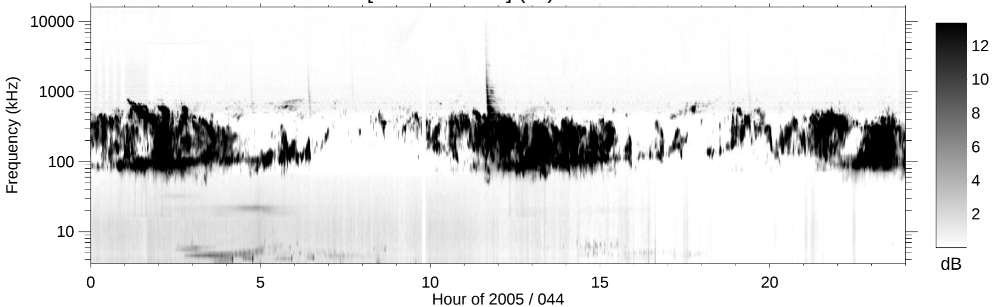
RPWS [ABCH1H2/Ex] (-B) 2005/02/13
