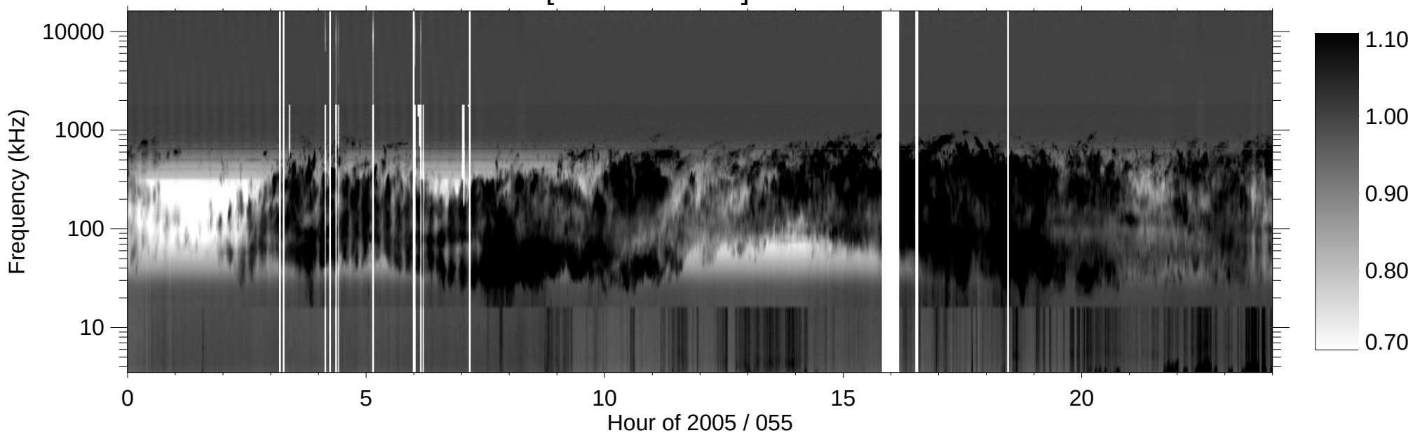
RPWS [ABCH1H2/Ex] (-B) 2005/02/24
