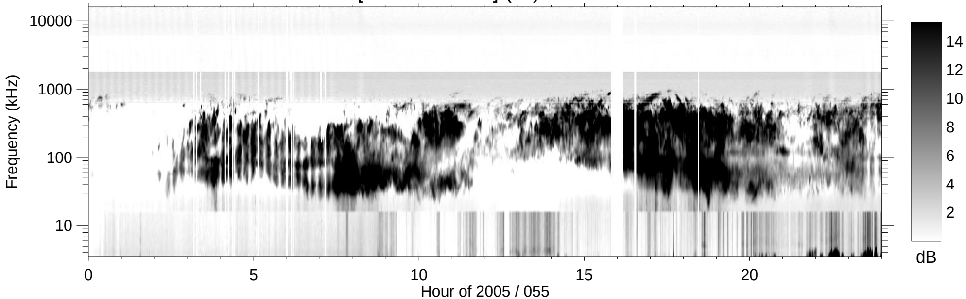
RPWS [ABCH1H2/Ex] (-B) 2005/02/24
