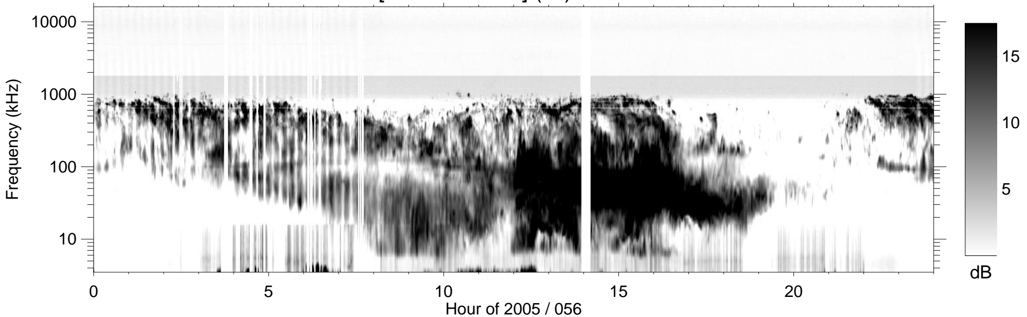
RPWS [ABCH1H2/Ex] (-B) 2005/02/25
