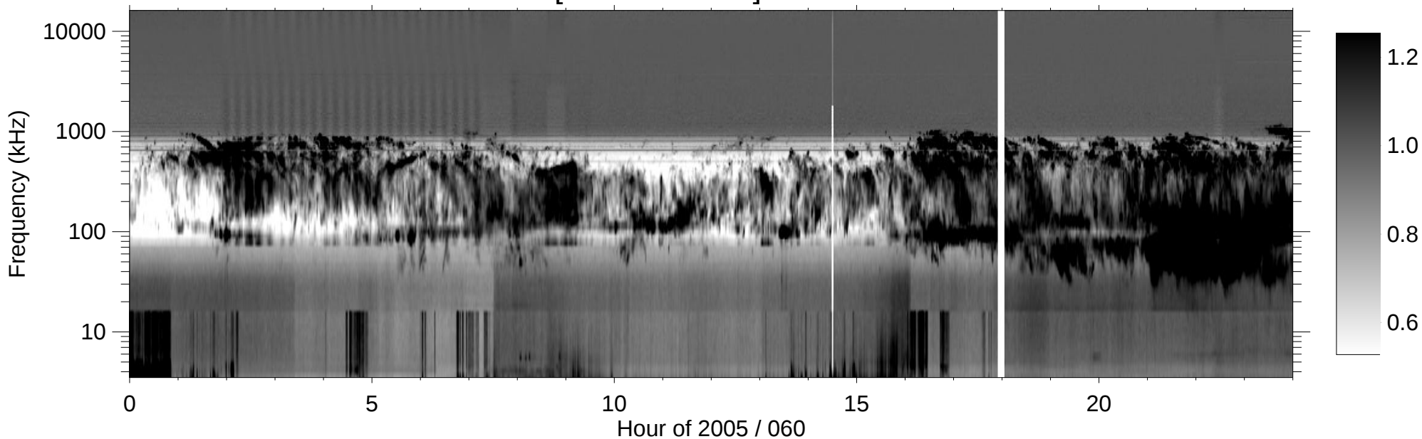
RPWS [ABCH1H2/Ex] (-B) 2005/03/01
