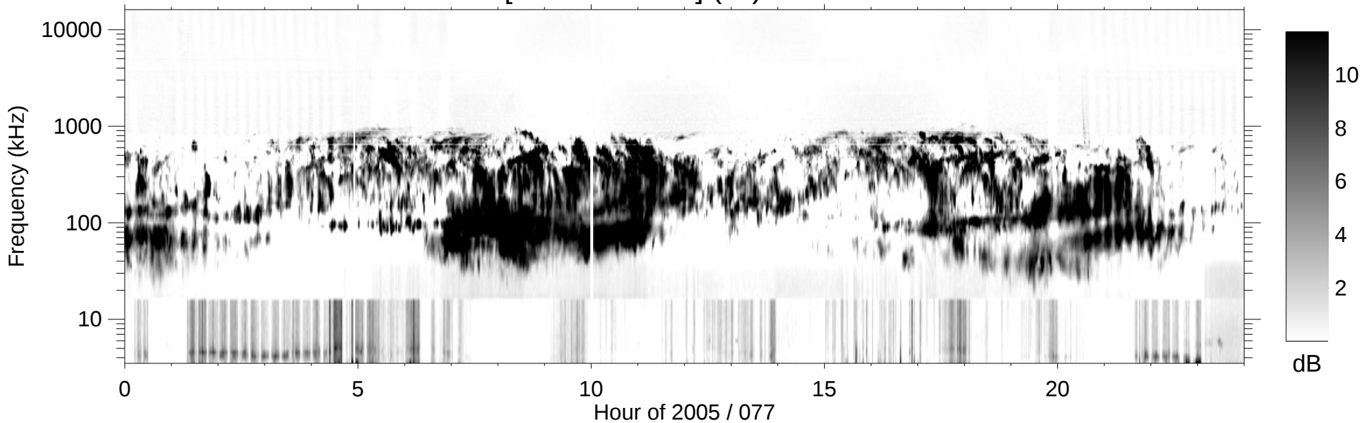
RPWS [ABCH1H2/Ex] (-B) 2005/03/18
