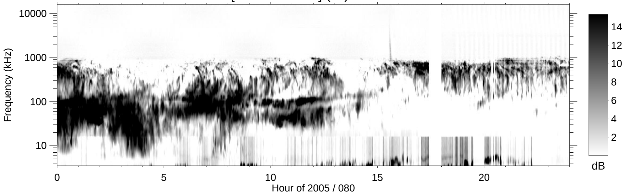
RPWS [ABCH1H2/Ex] (-B) 2005/03/21
