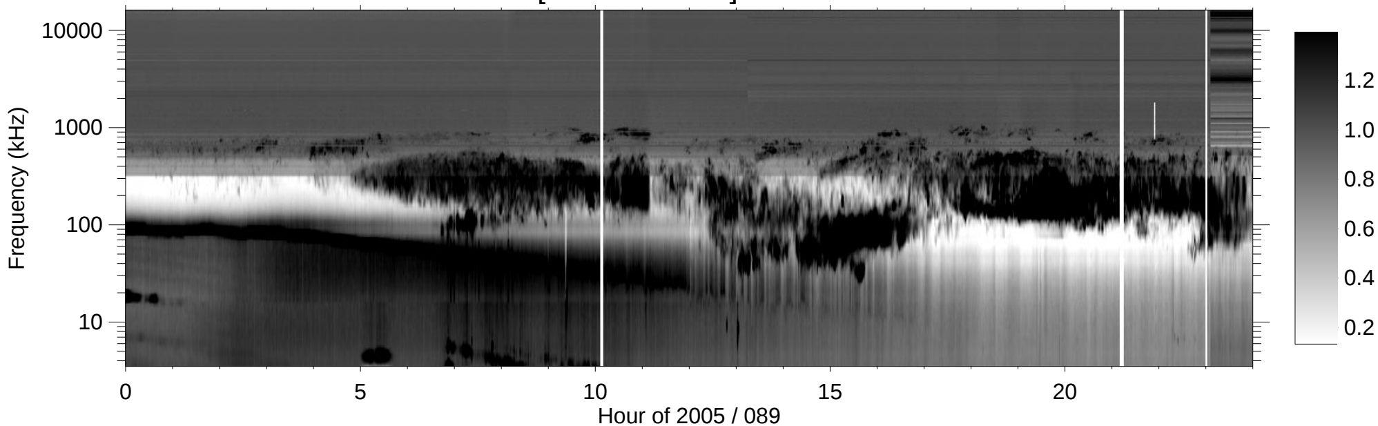
RPWS [ABCH1H2/Ex] (-B) 2005/03/30
