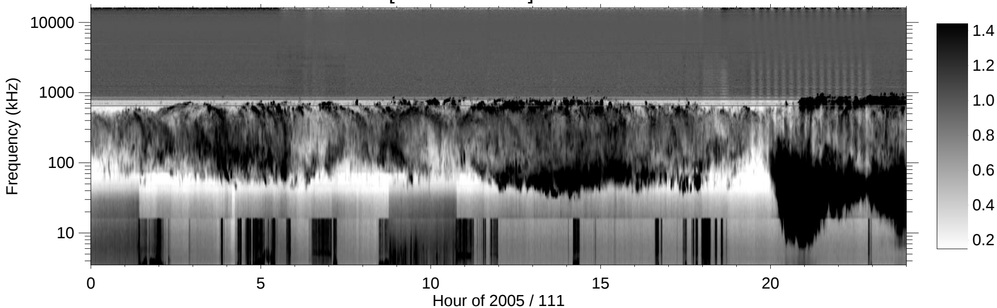
RPWS [ABCH1H2/Ex] (-B) 2005/04/21
