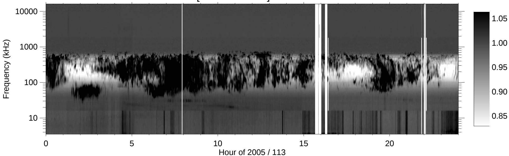
RPWS [ABCH1H2/Ex] (-B) 2005/04/23
