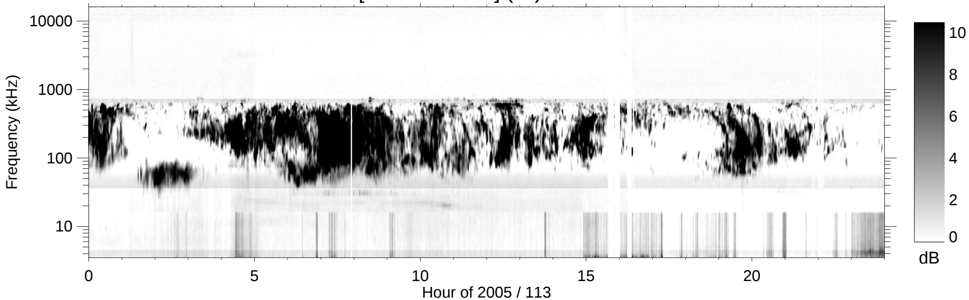
RPWS [ABCH1H2/Ex] (-B) 2005/04/23
