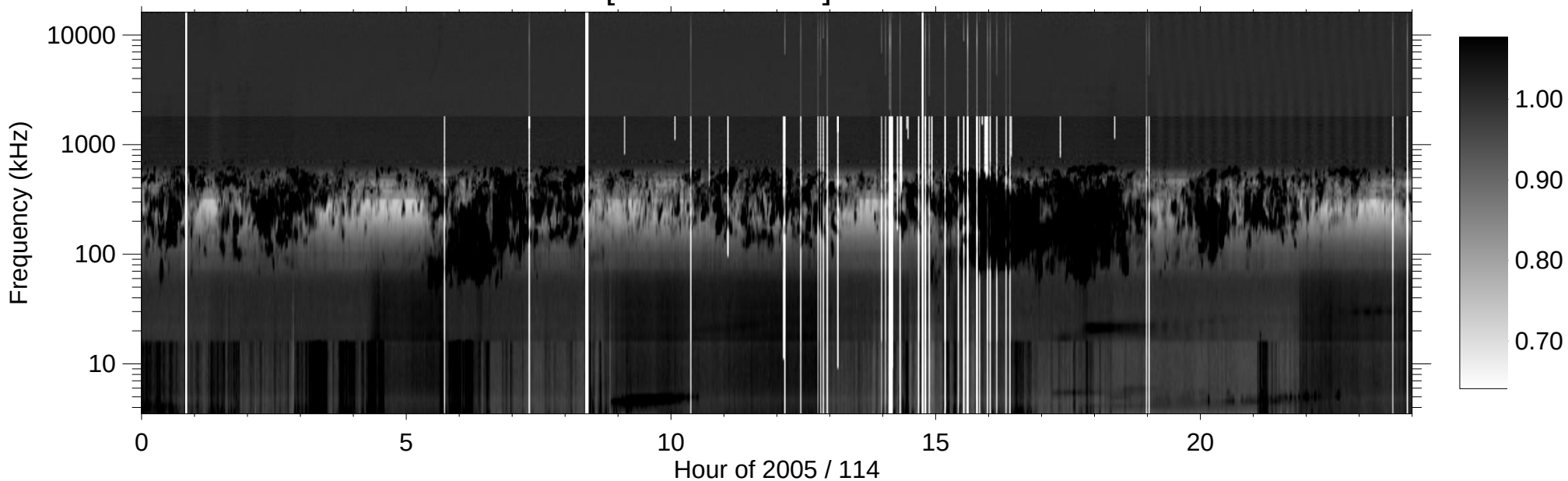
RPWS [ABCH1H2/Ex] (-B) 2005/04/24
