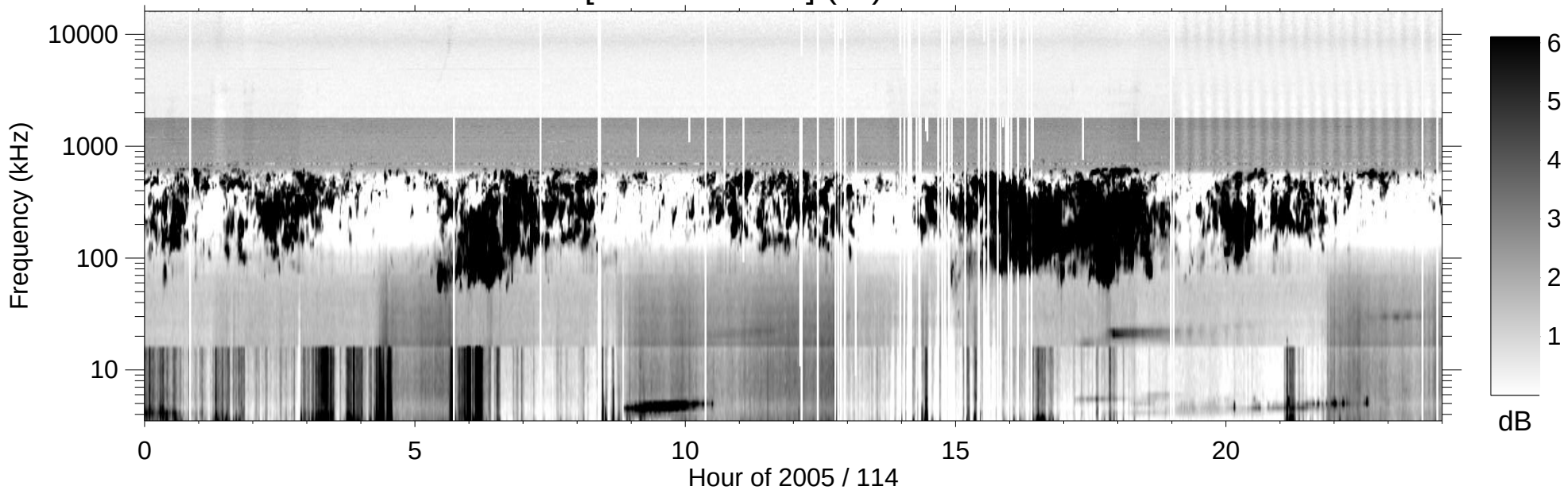
RPWS [ABCH1H2/Ex] (-B) 2005/04/24
