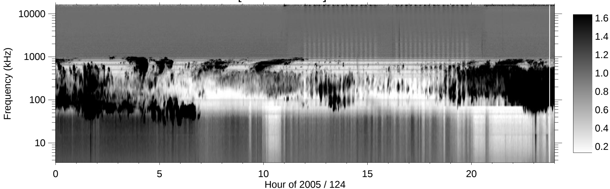
RPWS [ABCH1H2/Ex] (-B) 2005/05/04
