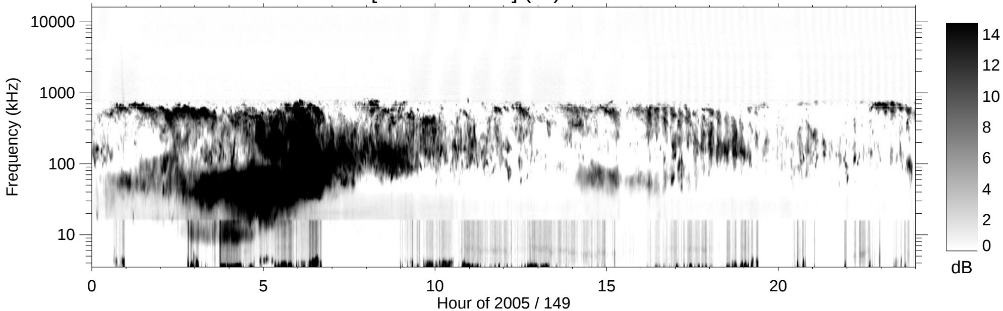
RPWS [ABCH1H2/Ex] (-B) 2005/05/29
