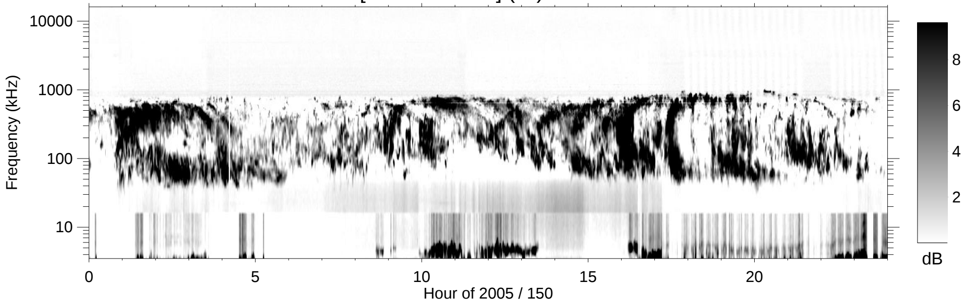
RPWS [ABCH1H2/Ex] (-B) 2005/05/30
