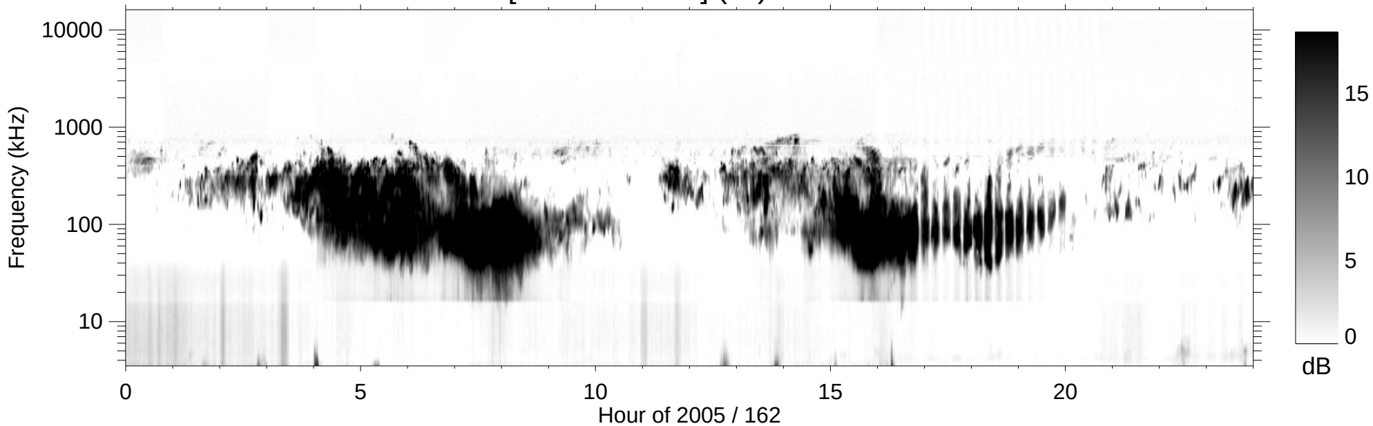
RPWS [ABCH1H2/Ex] (-B) 2005/06/11
