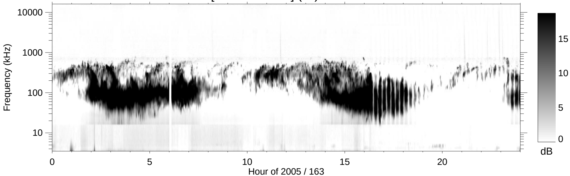
RPWS [ABCH1H2/Ex] (-B) 2005/06/12
