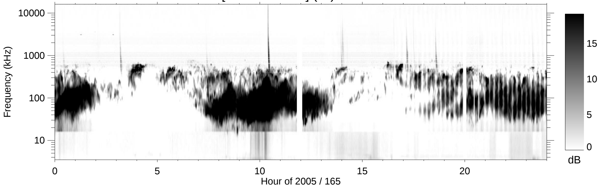
RPWS [ABCH1H2/Ex] (-B) 2005/06/14
