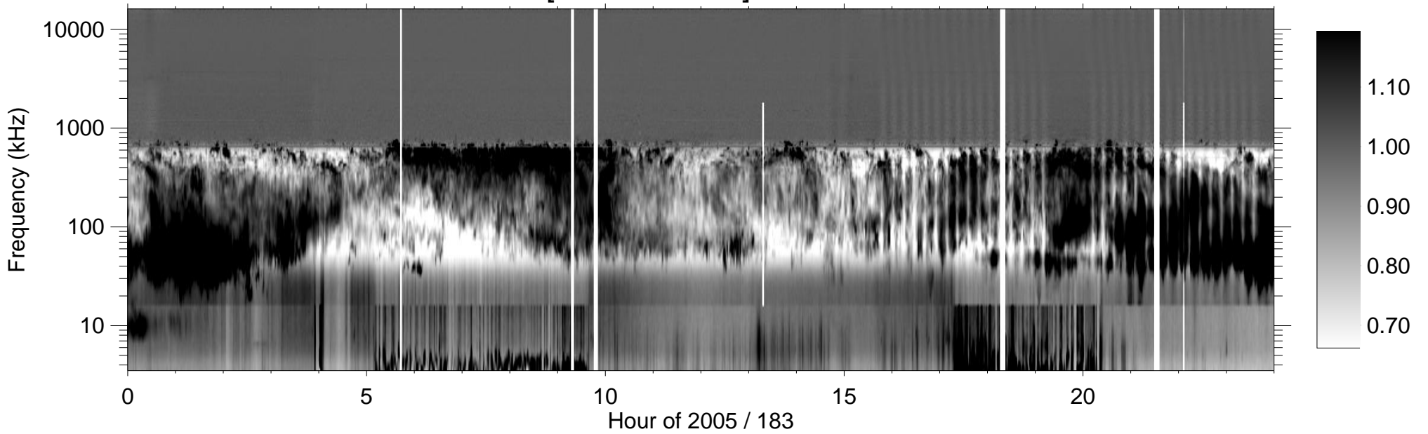
RPWS [ABCH1H2/Ex] (-B) 2005/07/02
