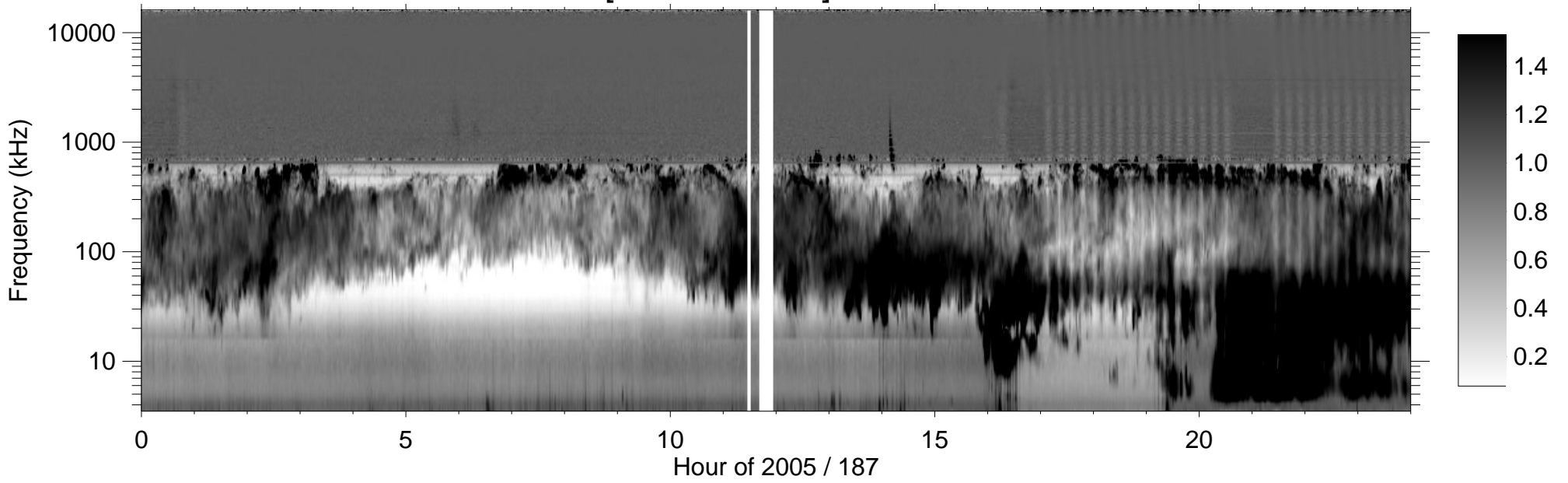
RPWS [ABCH1H2/Ex] (-B) 2005/07/06
