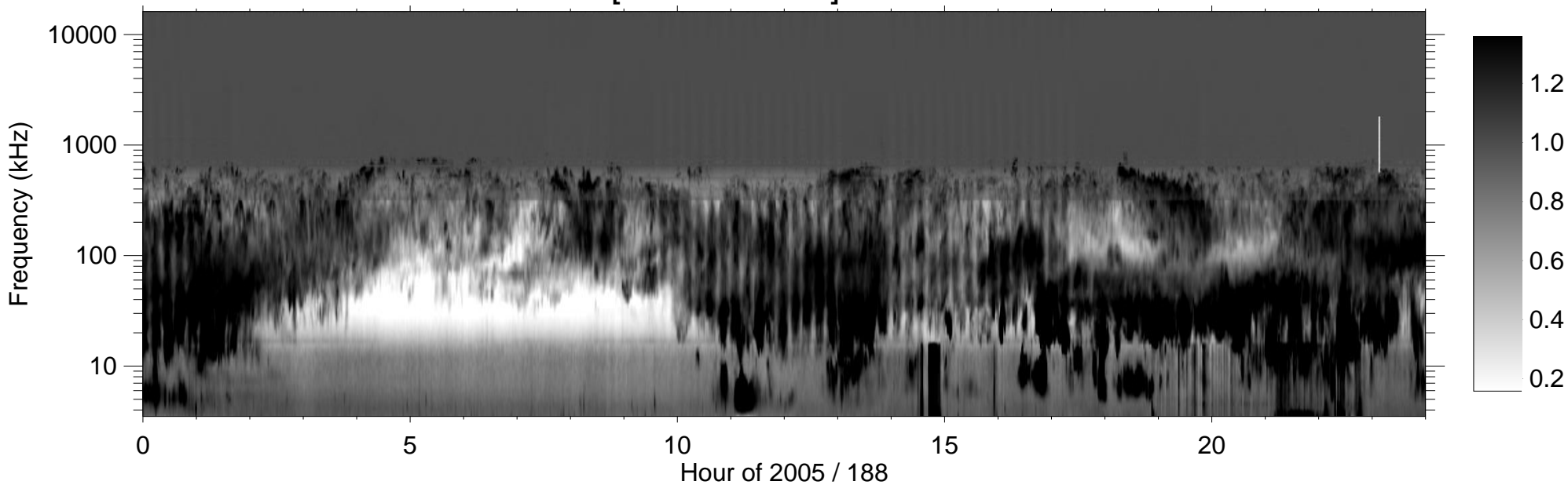
RPWS [ABCH1H2/Ex] (-B) 2005/07/07
