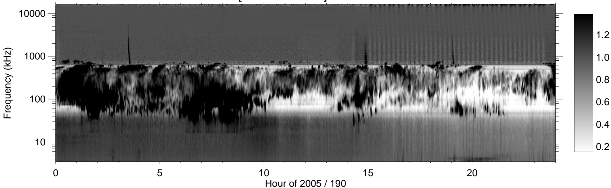
RPWS [ABCH1H2/Ex] (-B) 2005/07/09
