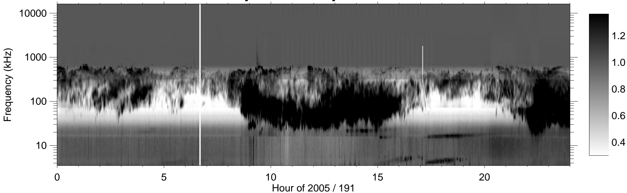
RPWS [ABCH1H2/Ex] (-B) 2005/07/10
