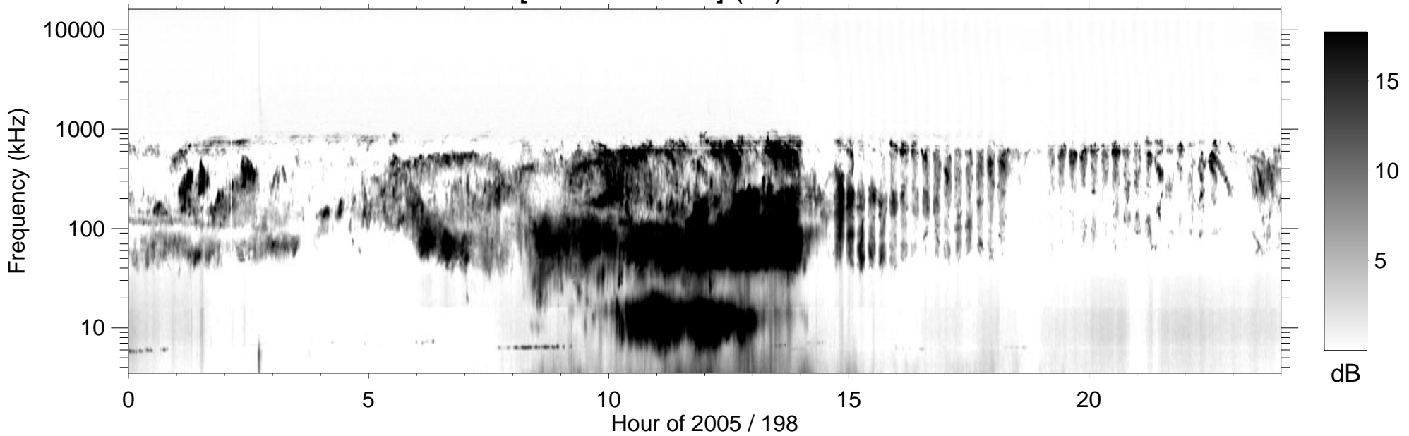
RPWS [ABCH1H2/Ex] (-B) 2005/07/17
