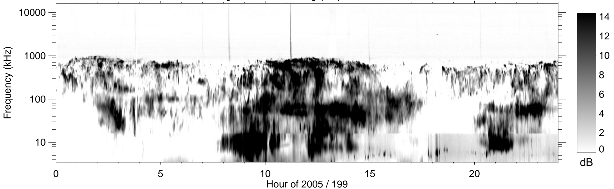
RPWS [ABCH1H2/Ex] (-B) 2005/07/18
