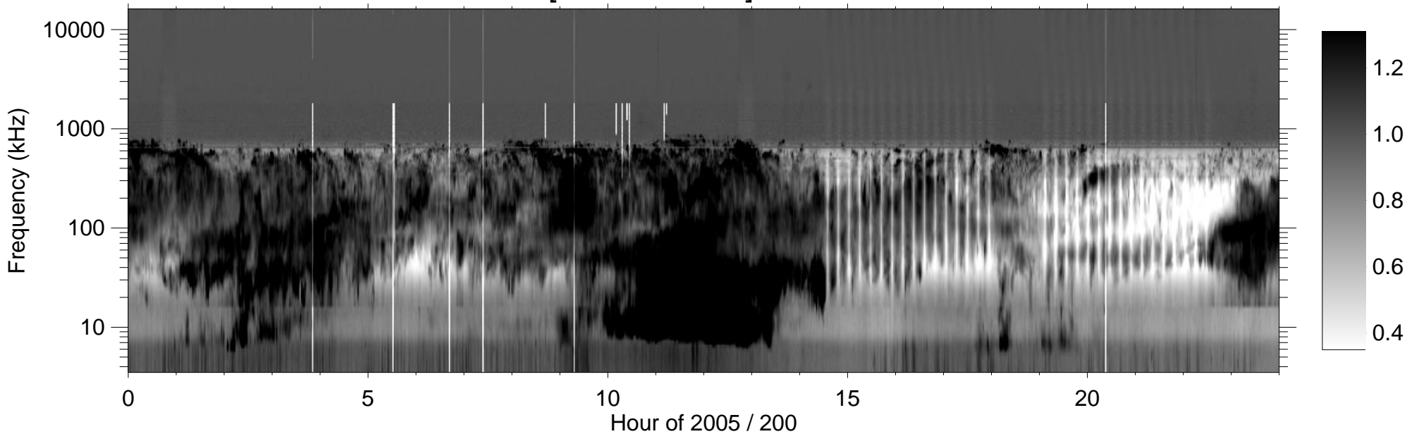
RPWS [ABCH1H2/Ex] (-B) 2005/07/19
