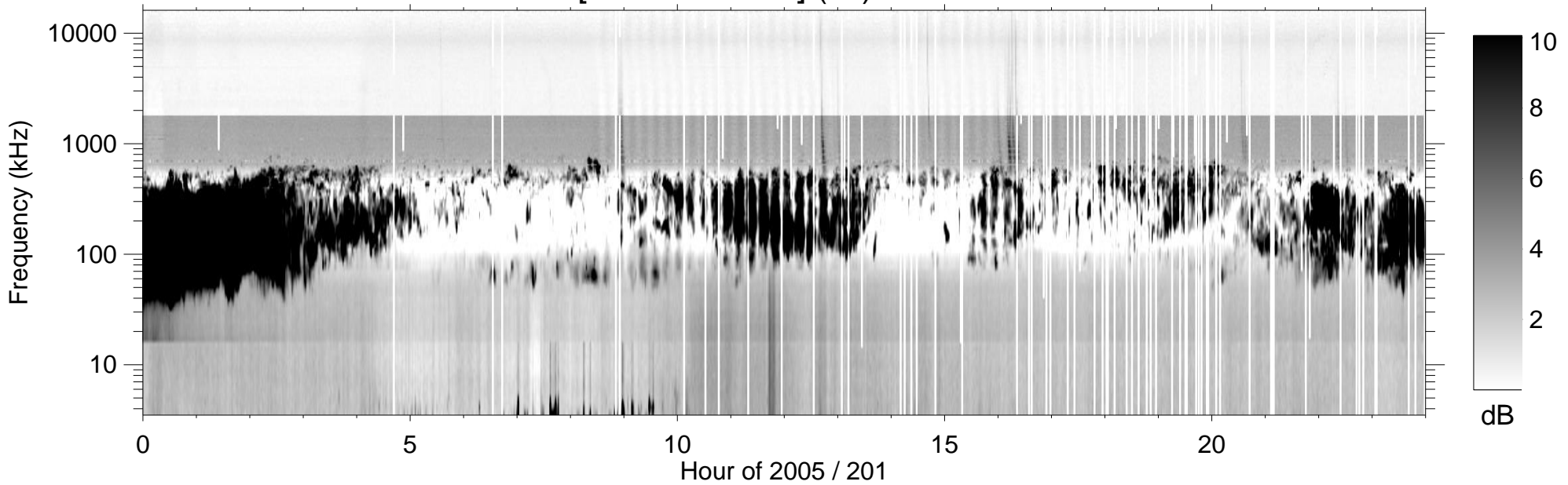
RPWS [ABCH1H2/Ex] (-B) 2005/07/20
