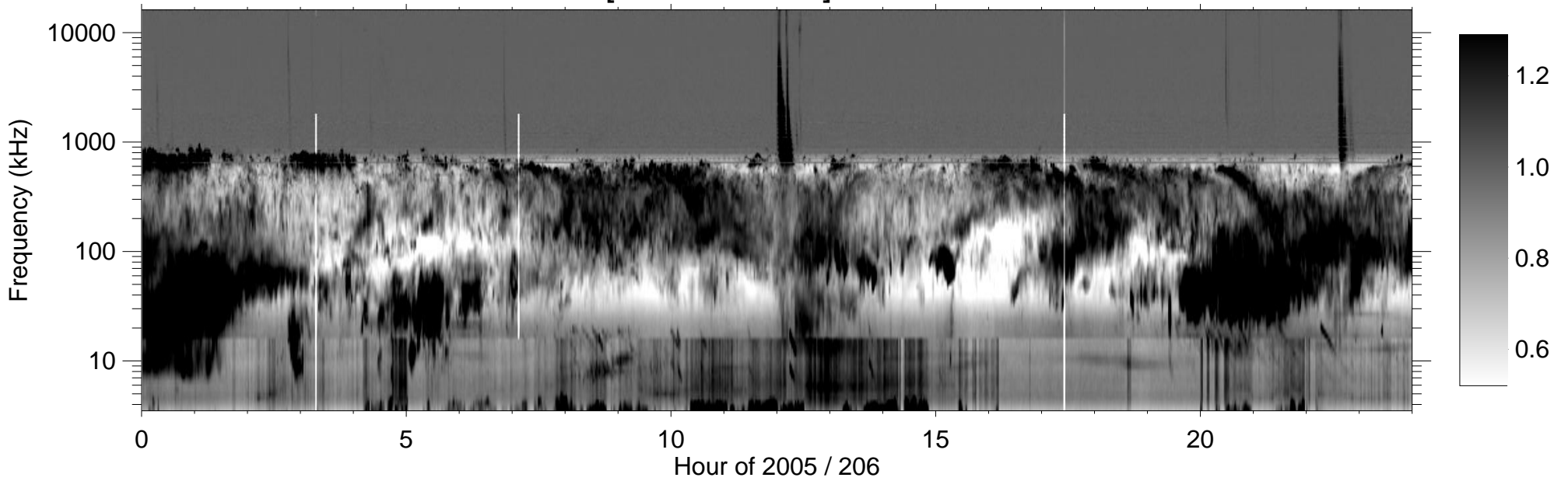
RPWS [ABCH1H2/Ex] (-B) 2005/07/25
