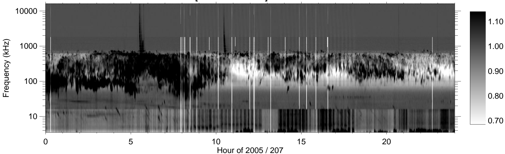
RPWS [ABCH1H2/Ex] (-B) 2005/07/26
