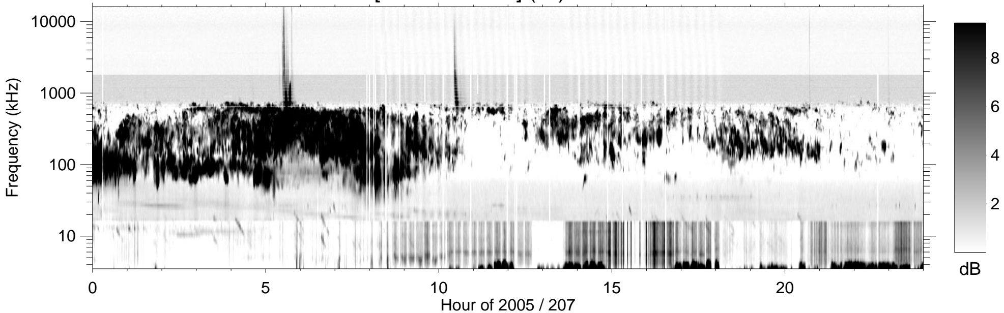
RPWS [ABCH1H2/Ex] (-B) 2005/07/26
