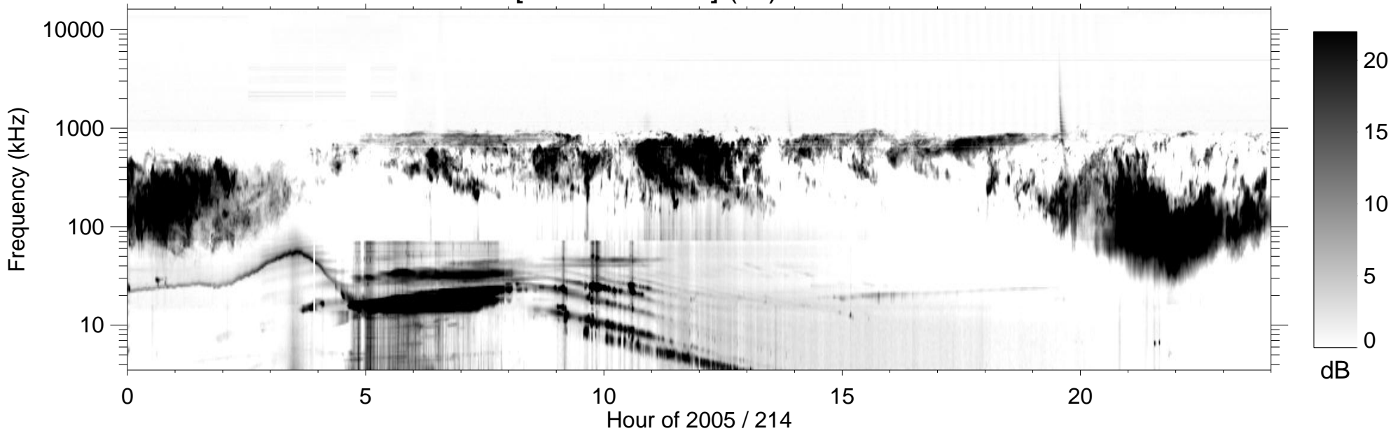
RPWS [ABCH1H2/Ex] (-B) 2005/08/02
