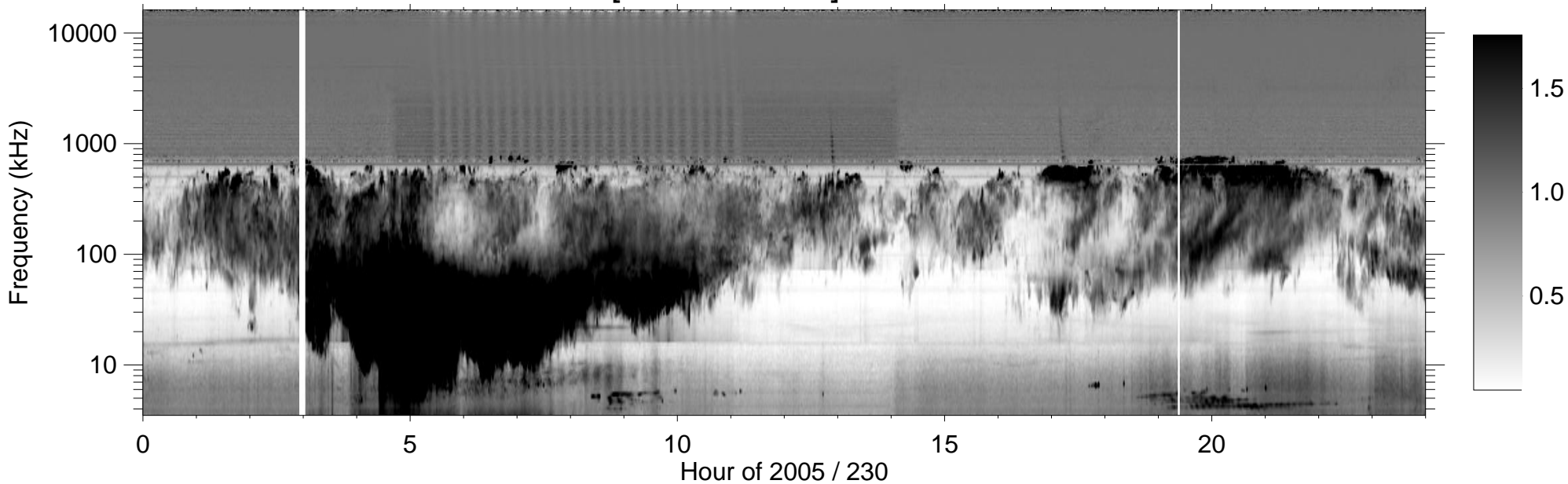
RPWS [ABCH1H2/Ex] (-B) 2005/08/18
