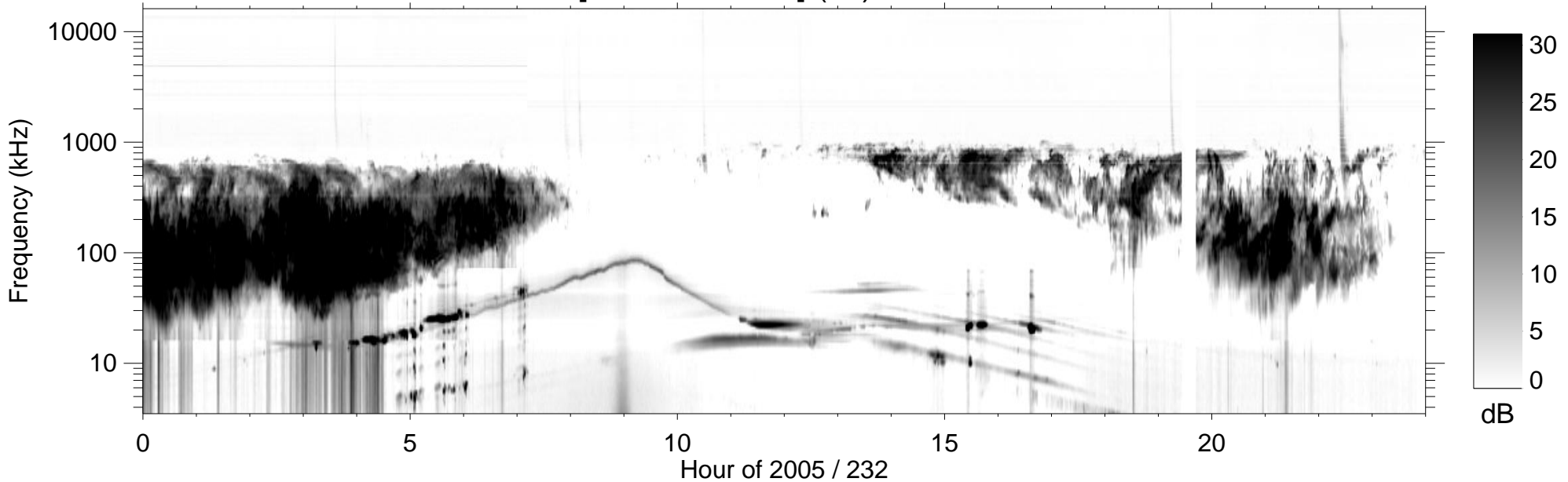
RPWS [ABCH1H2/Ex] (-B) 2005/08/20
