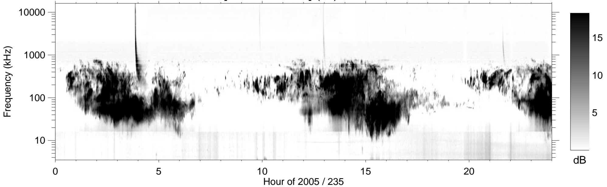
RPWS [ABCH1H2/Ex] (-B) 2005/08/23
