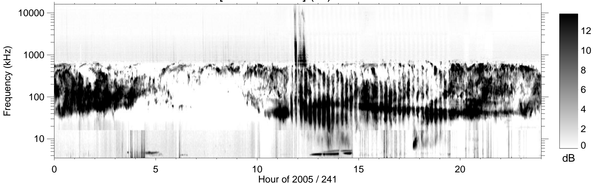
RPWS [ABCH1H2/Ex] (-B) 2005/08/29
