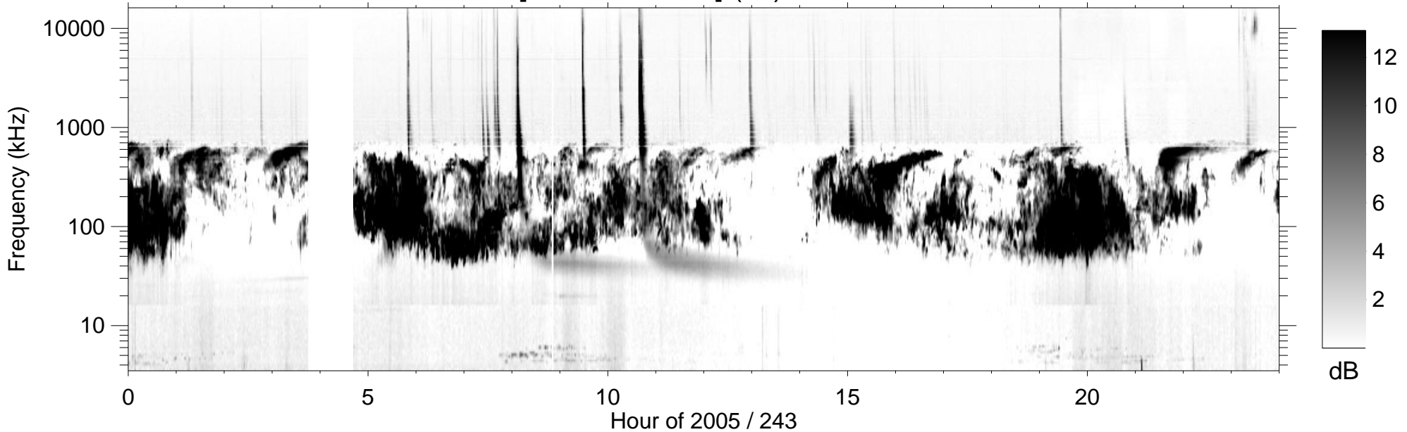
RPWS [ABCH1H2/Ex] (-B) 2005/08/31
