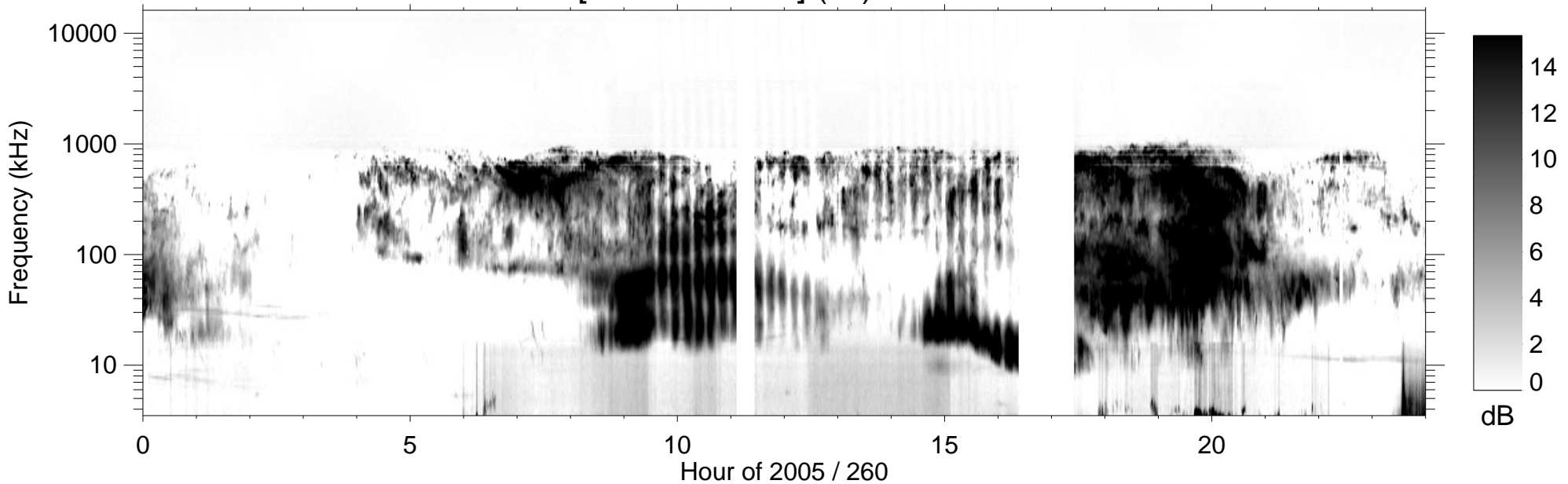
RPWS [ABCH1H2/Ex] (-B) 2005/09/17
